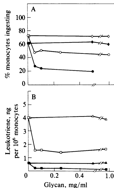
FIG. 2. Dose-dependent effects of pretreatment with soluble \beta -glucan (○, ●) and mannan (◇, ◆) on the percentages of adherent monocytes subsequently ingesting \geq 1 glucan particle at inputs of 2.2 \times 10^6 per ml (●, ◆) and 8.6 \times 10^6 per ml (○, ◇) (A) and dose-dependent effects of pretreatment with \beta -glucan (□, ■) and mannan (Δ, ▲) on the subsequent release of immunoreactive LTB 4 (□, Δ) and LTC 4 (■, ▲) by 8.6 \times 10^6 glucan particles per ml (B). The data represent a single experiment performed simultaneously with monocytes from the same donor used for the study depicted in Fig. 3.
