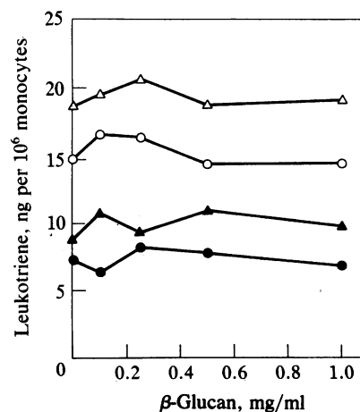
FIG. 5. Dose-dependent effects of \beta -glucan pretreatment of adherent monocytes from two separate donors on the subsequent release of LTB 4 ( \triangle , \circ ) and LTC 4 ( \blacktriangle , \bullet ) with 2.5 \mu M calcium ionophore A23187.
