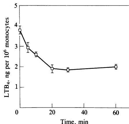
FIG. 4. Time-dependent effects of pretreatment of adherent monocytes with 100 \mu g of soluble \beta -glucan per ml on their subsequent release of LTB 4 ( \square ) after a 40-min incubation with 8.6 \times 10^6 glucan particles per ml. The data are the mean of duplicate determinations in a single experiment.
