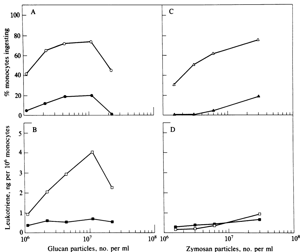
FIG. 1. Dose-dependent effects of glucan particles and zymosan particles on the capacity of adherent monocytes from the same donor to phagocytose \geq 1 (○) and \geq 3 (●) glucan particles (A) or \geq 1 (Δ) and \geq 3 (▲) zymosan particles (C) and dose effects on the release of immunoreactive LTB 4 (□) and LTC 4 (●) in response to glucan (B) or zymosan (D) particles. The phagocytic data are expressed as the percentage of ingesting monocytes in single determinations on coverslips and the leukotriene measurements are plotted as mean ng per 10^6 monocytes from duplicates on Petri dishes.
